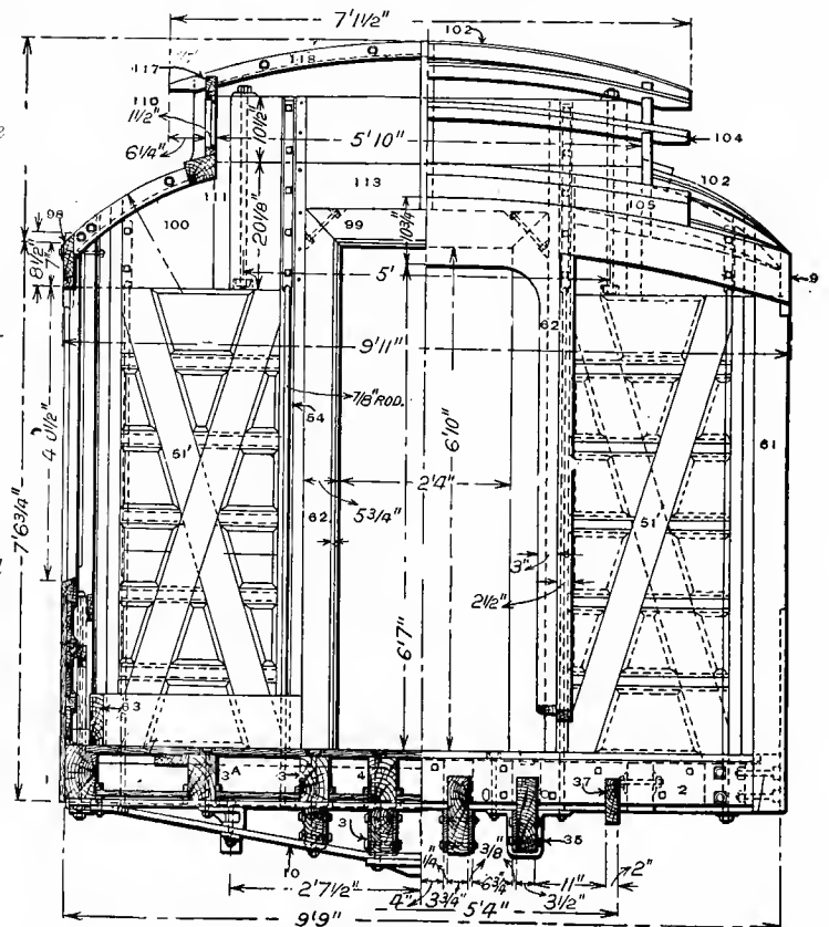
Fig. 539a. End Elevation of Framing. FIRST CLASS PASSENGER COACH. (Full Framing is Shown in Figs. 419-427.)
